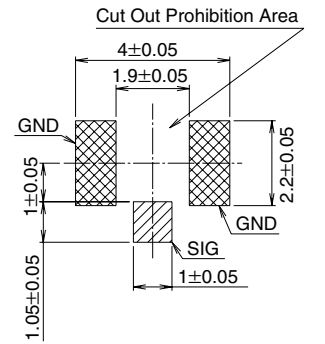
Recommended PCB mounting pattern
