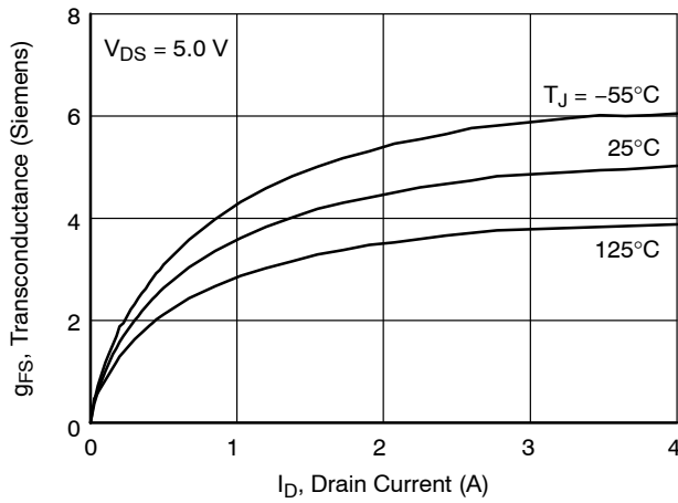
Figure 13. Transconductance Variation with Drain Current and Temperature
