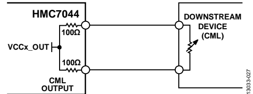
Figure 33. DC-Coupled CML (Internal) Output Driver
